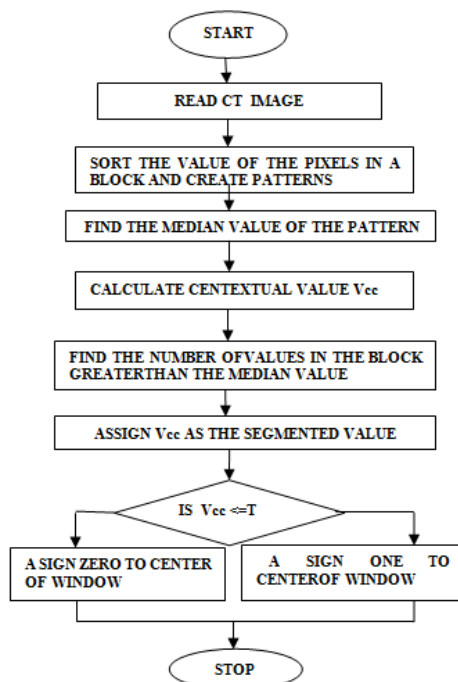
Fig. 2 Flow diagram of proposed algorithm
